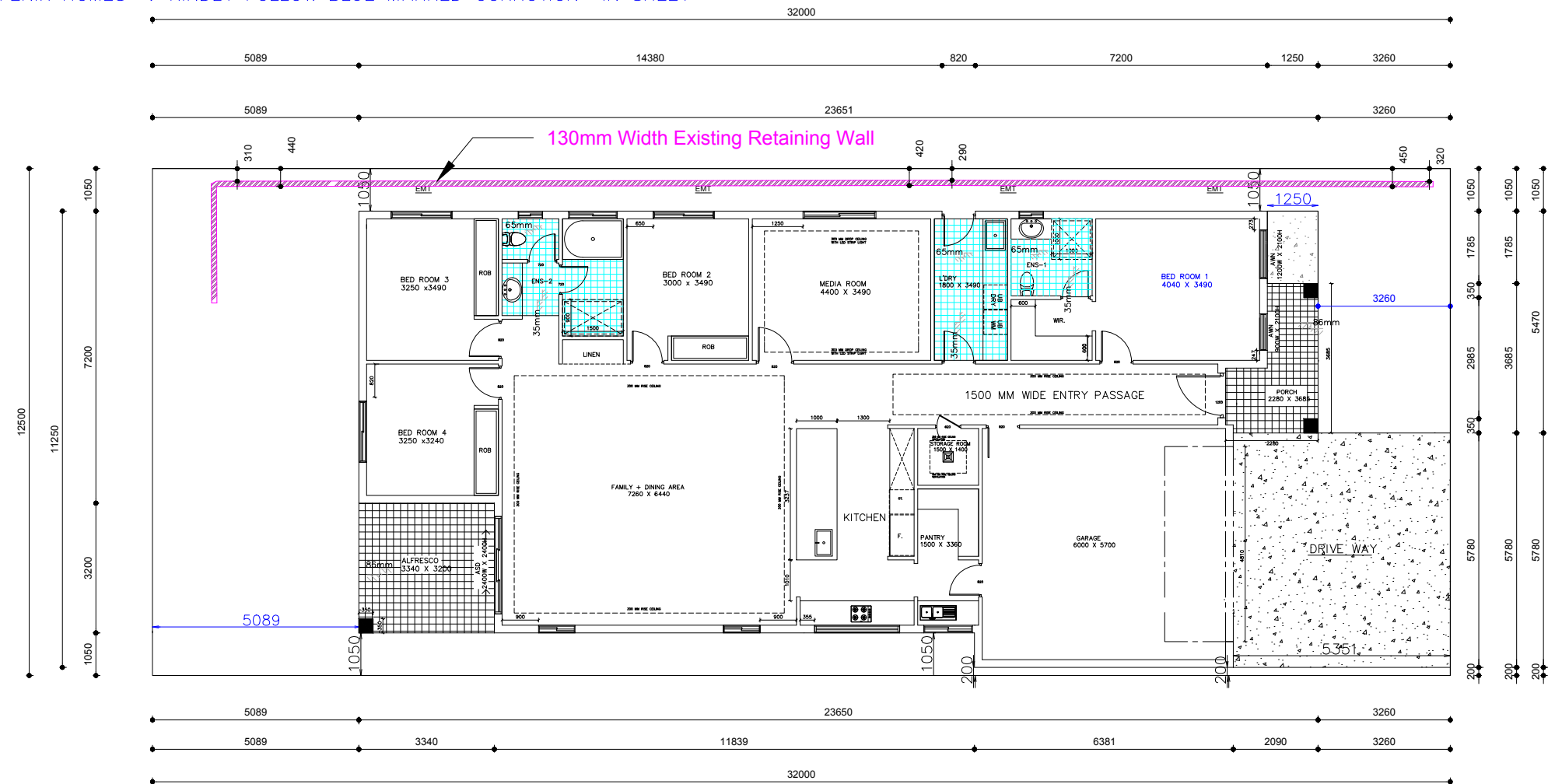
PROPOSED SLAB SETOUT PLAN SCALE 1:100
